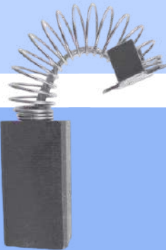
Escobilla NR-010 Medidas 1.250 x 0.630 x 0.394 in G
